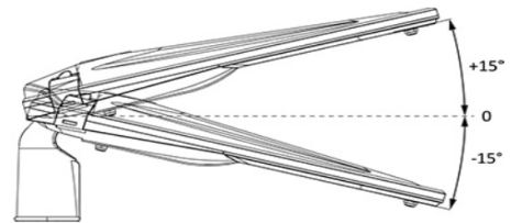
Vertical installation: Adjustable tilt angle: 0-5-10-15°
