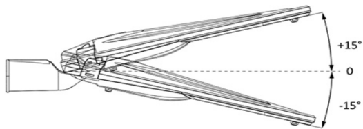
Horizontal installation: Adjustable tilt angle: 0-5-10-15°
